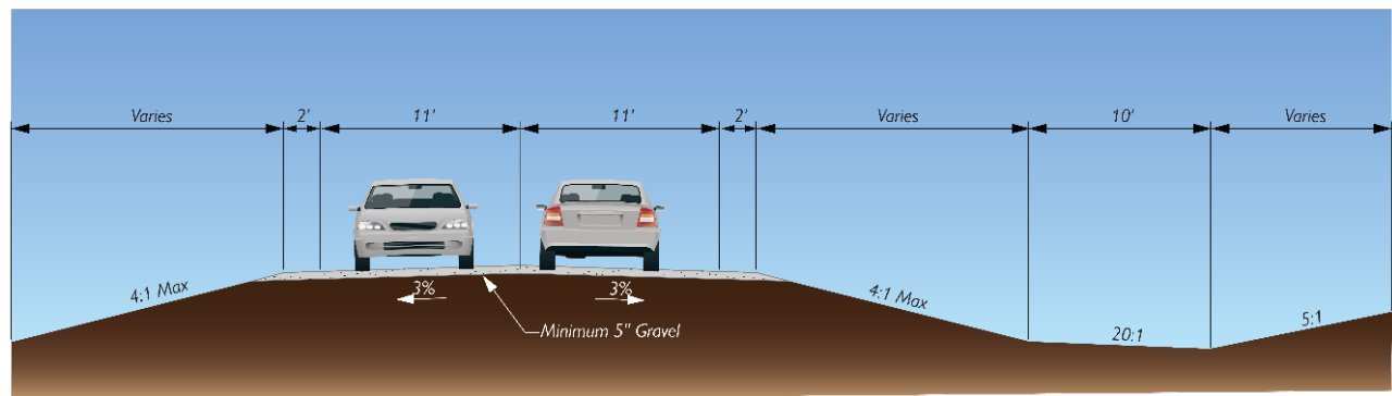
Base Typical Cross Section – Unpaved
